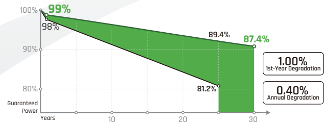
Sonnex TOPCon Dual Glass Module Performance Warranty
