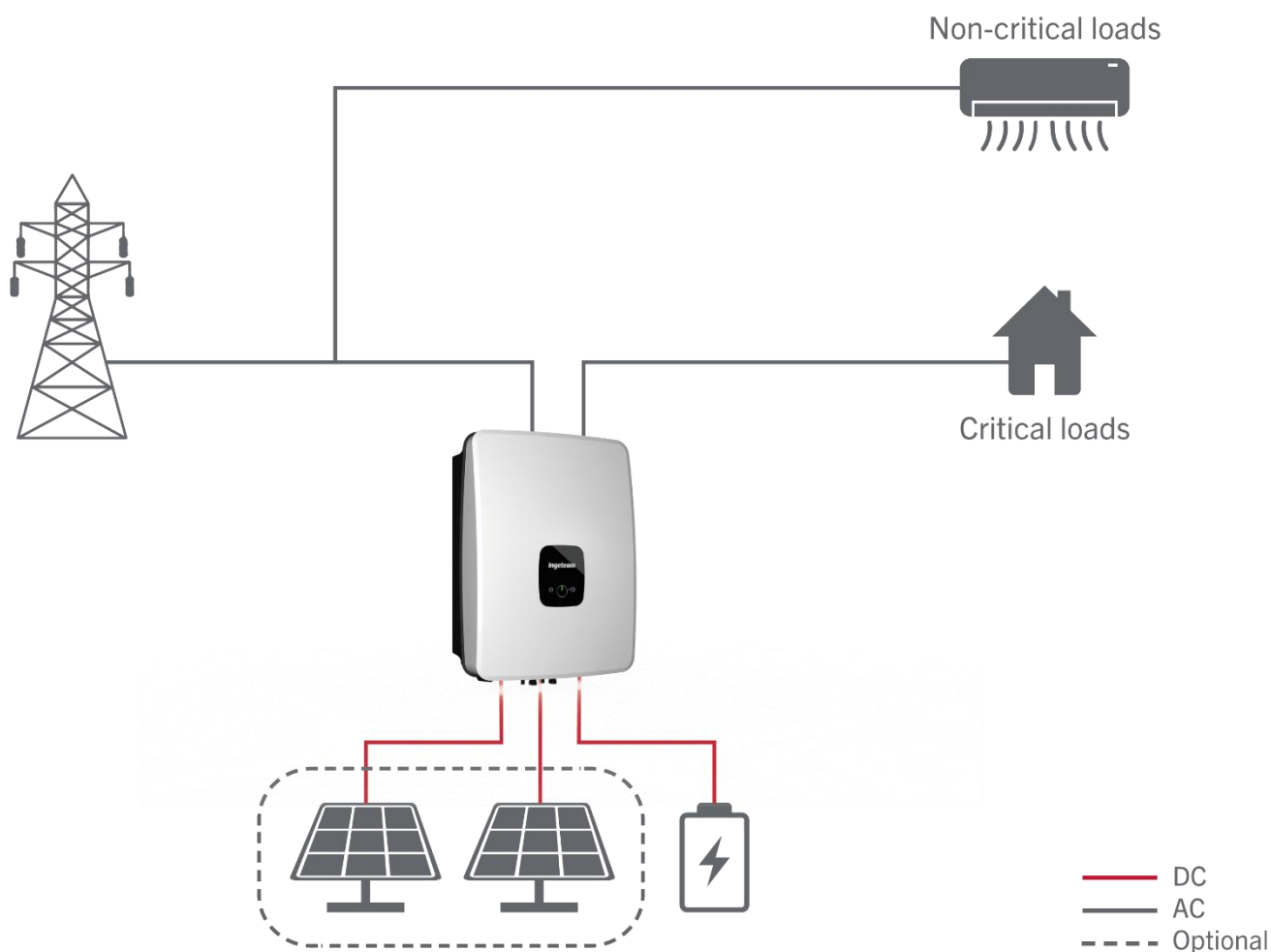
Figure 3: UPS installation
