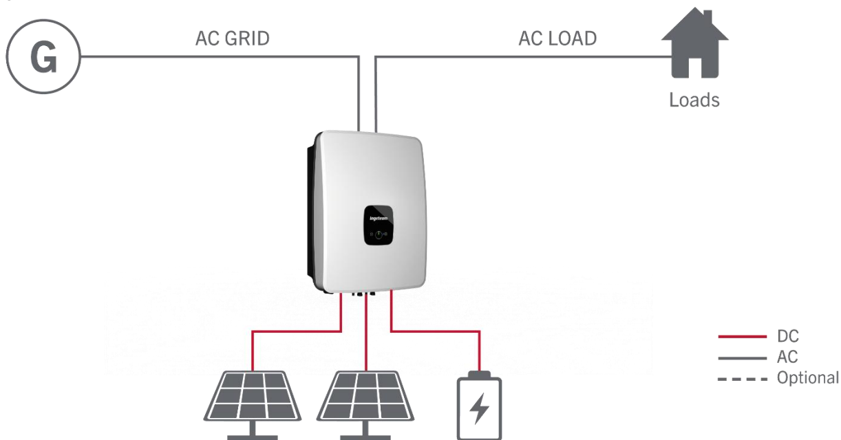
Figure 4: Stand-alone installation
