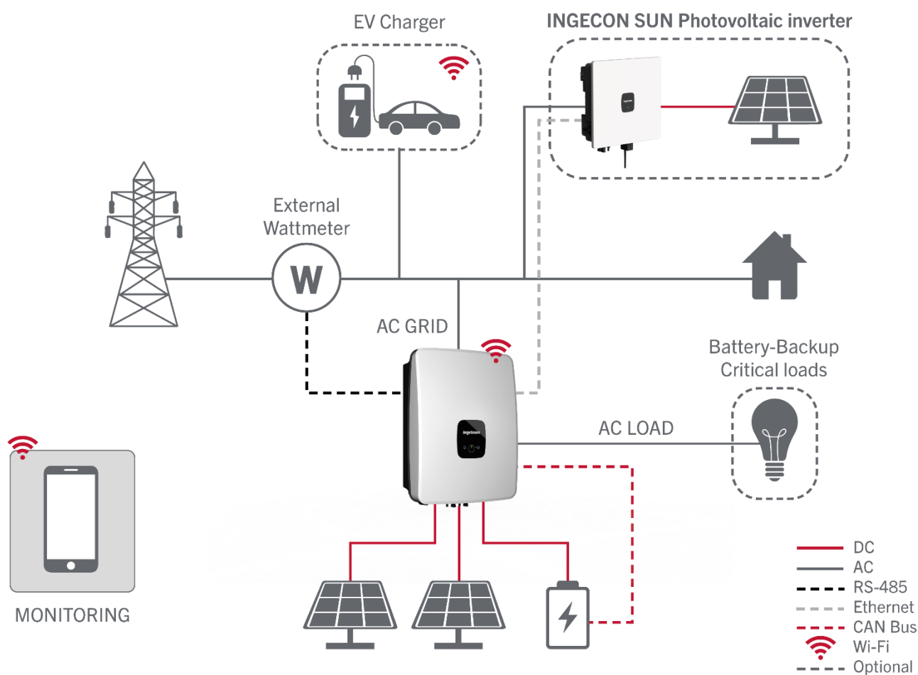
Figure 2: Self-consumption installation
