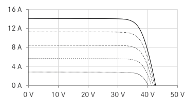
UI-diagram e.g. LX-470M/182-120+
