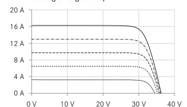
UP-diagram e.g. 460 Wp
