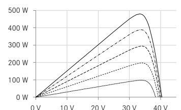
UP-diagram e.g. 480 Wp
