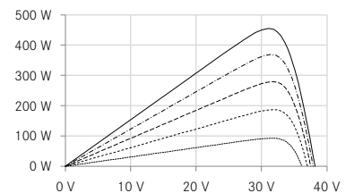
UP-diagram e.g. 455 Wp
