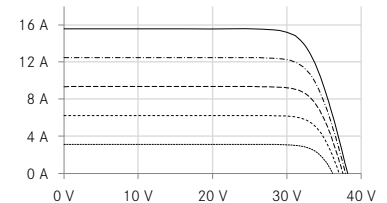
UP-diagram e.g. 455 Wp
