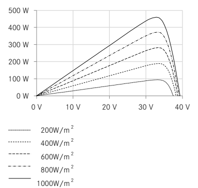
UP-diagram e.g. 460 Wp
