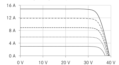
UP-diagram e.g. 460 Wp
