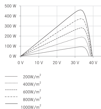
UP-diagram e.g. 460 Wp
