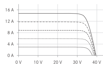
UP-diagram e.g. 460 Wp
