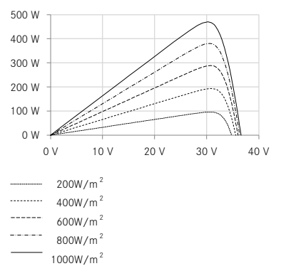
UP-diagram e.g. 470 Wp
