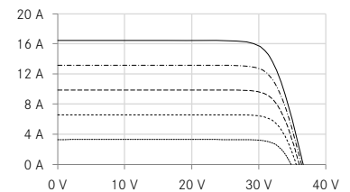
UP-diagram e.g. 470 Wp
