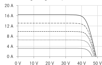
UP-diagram e.g. 630 Wp
