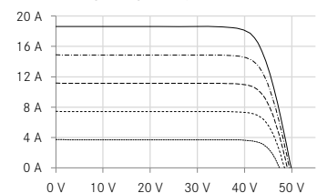
UP-diagram e.g. 720 Wp
