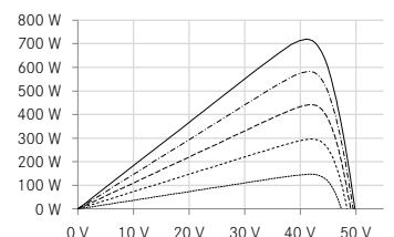
UP-diagram e.g. 720 Wp
