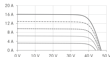
UI - diagram e.g. 600 Wp
