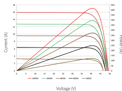
Characteristic curves (615W)
