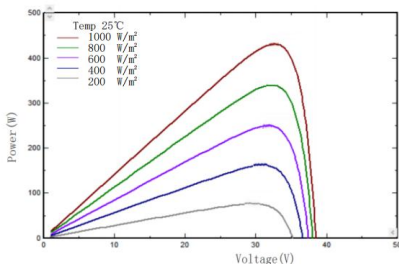
I-V/P-V Curve at Different Irradiation (435W)
