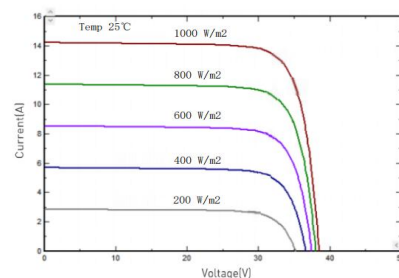
I-V/P-V Curve at Different Irradiation (435W)
