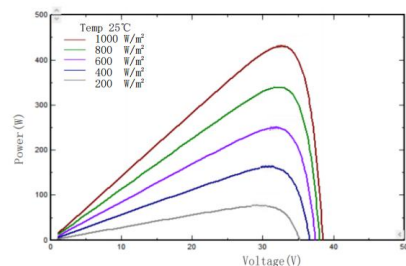
I-V/P-V Curve at Different Irradiation (435W)
