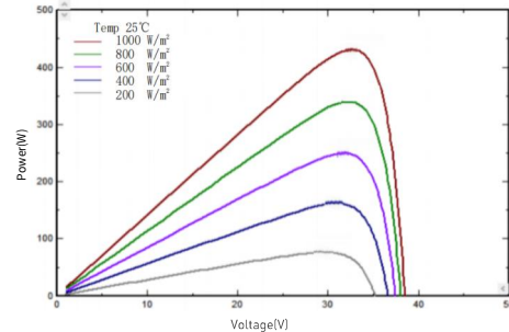
I-V/P-V Curve at Different Irradiation (455W)
