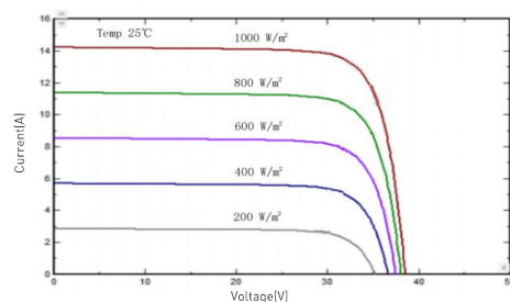
I-V/P-V Curve at Different Irradiation (455W)
