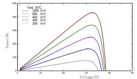
I-V/P-V Curve at Different Irradiation (450W)
