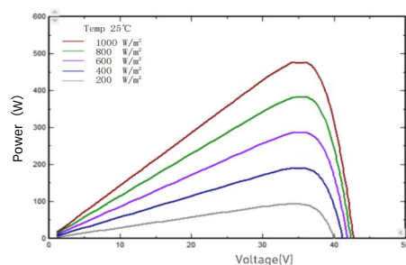
I-V/P-V Curve at Different Irradiation (485W)
