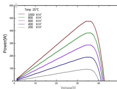
I-V/P-V Curve at Different Irradiation (500W)
