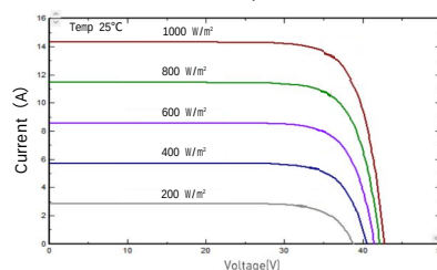
I-V/P-V Curve at Different Irradiation (500W)
