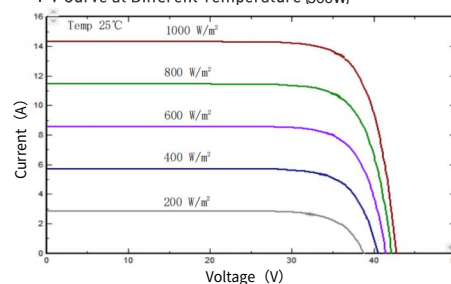
I-V/P-V Curve at Different Irradiation 500W
