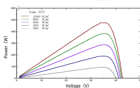
I-V/P-V Curve at Different Irradiation 500W
