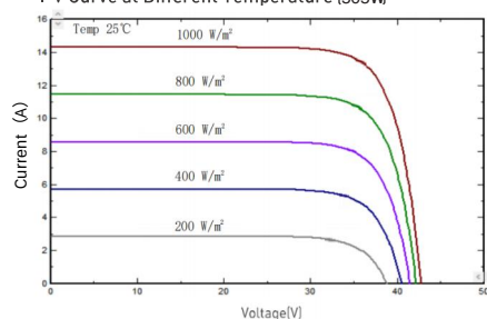
I-V/P-V Curve at Different Irradiation (505W)
