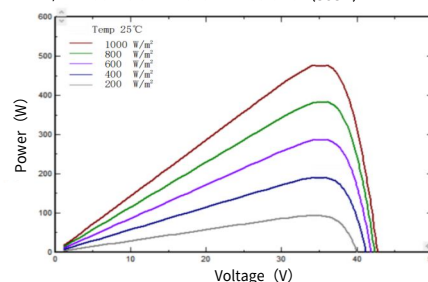
I-V/P-V Curve at Different Irradiation (505W)
