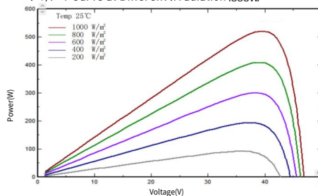
I-V/P-V Curve at Different Irradiation (555W)
