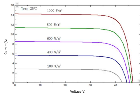
I-V/P-V Curve at Different Irradiation (555W)
