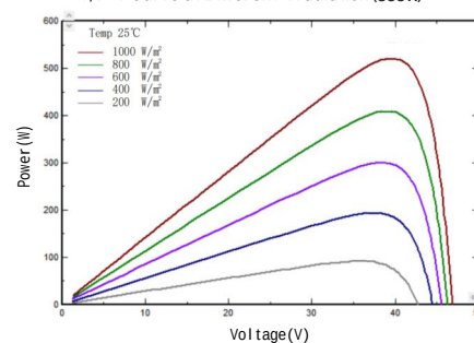
I-V/P-V Curve at Different Irradiation (555W)
