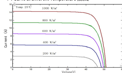
I-V/P-V Curve at Different Irradiation [580W]
