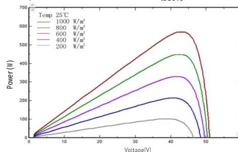
I-V/P-V Curve at Different Irradiation [580W]
