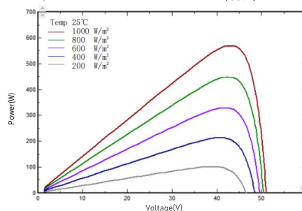
I-V/P-V Curve at Different Irradiation (580W)
