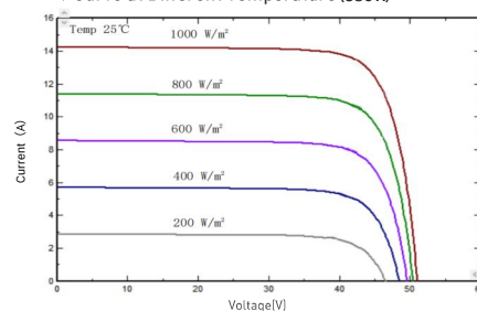
I-V/P-V Curve at Different Irradiation (580W)
