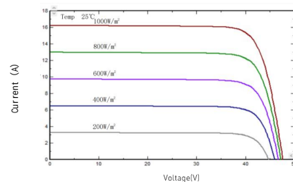
I-V/P-V Curve at Different Irradiation [605W]
