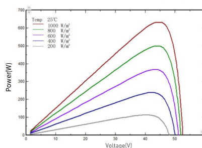
I-V/P-V Curve at Different Irradiation (630W)
