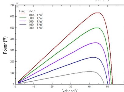
I-V/P-V Curve at Different Irradiation [630W]
