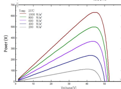
I-V/P-V Curve at Different Irradiation [655W]
