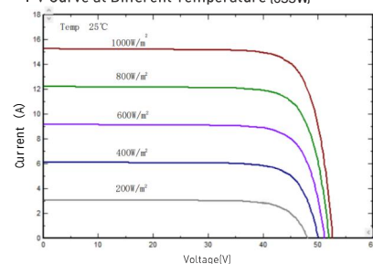
I-V/P-V Curve at Different Irradiation [655W]
