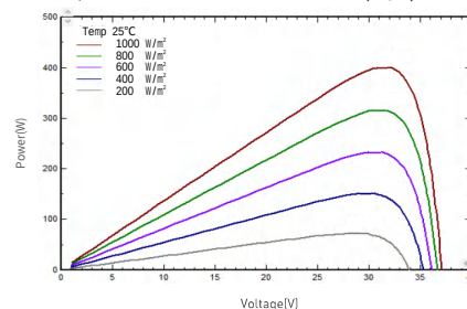
I-V/P-V Curve at Different Irradiation (410W)
