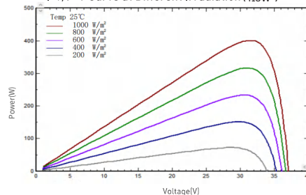
I-V/P-V Curve at Different Irradiation (410W)
