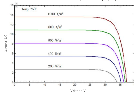
I-V/P-V Curve at Different Irradiation (410W)
