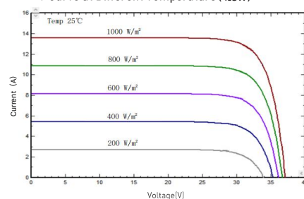
I-V/P-V Curve at Different Irradiation (415W)
