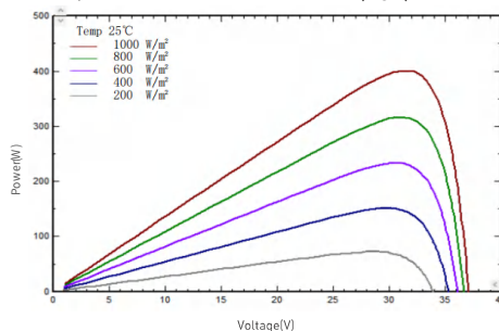
I-V/P-V Curve at Different Irradiation (415W)
