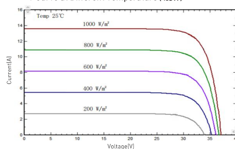
I-V/P-V Curve at Different Irradiation (415W)
