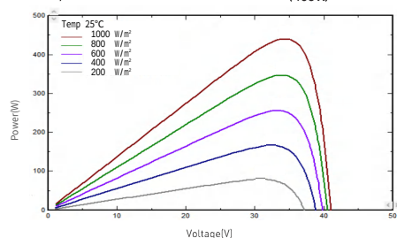
I-V/P-V Curve at Different Irradiation (460W)
