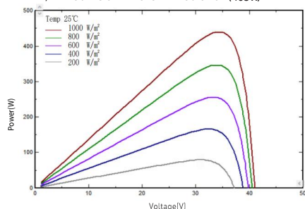
I-V/P-V Curve at Different Irradiation (465W)
