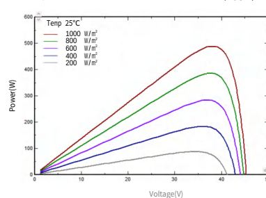
I-V/P-V Curve at Different Irradiation (495W)
