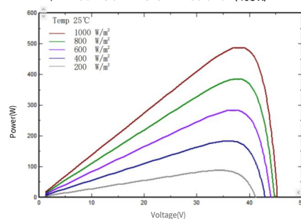
I-V/P-V Curve at Different Irradiation (495W)
