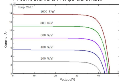
I-V/P-V Curve at Different Irradiation (495W)
