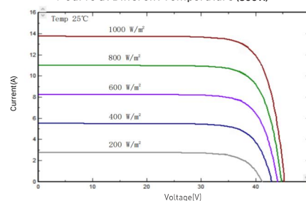
I-V/P-V Curve at Different Irradiation (500W)
