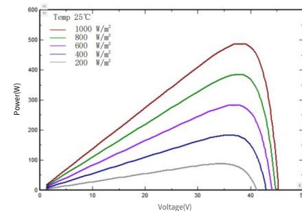
I-V/P-V Curve at Different Irradiation (500W)
