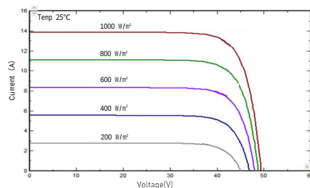
I-V/P-V Curve at Different Irradiation (550W)
