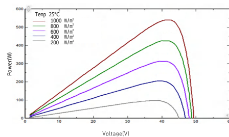
I-V/P-V Curve at Different Irradiation (550W)
