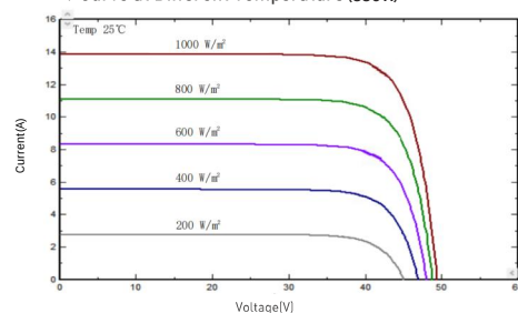
I-V/P-V Curve at Different Irradiation (550W)
