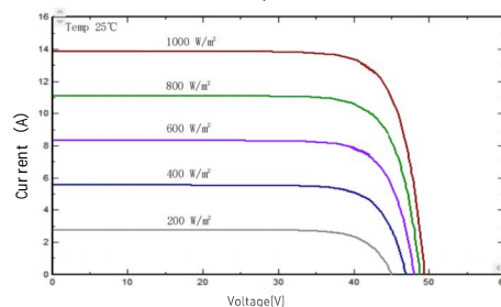
I-V/P-V Curve at Different Irradiation (555W)
