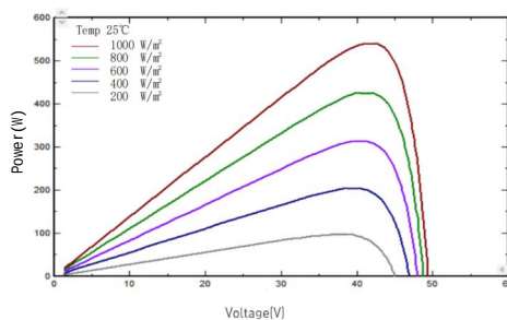
I-V/P-V Curve at Different Irradiation (555W)
