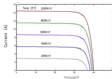
I-V/P-V Curve at Different Irradiation (460W)
