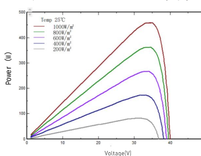
I-V/P-V Curve at Different Irradiation (470W)
