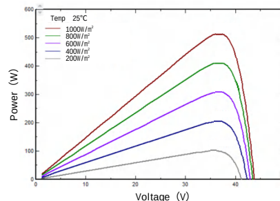
I-V/P-V Curve at Different Irradiation (520W)
