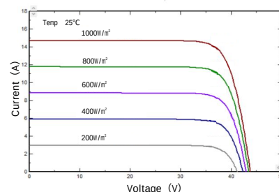
I-V/P-V Curve at Different Irradiation (520W)
