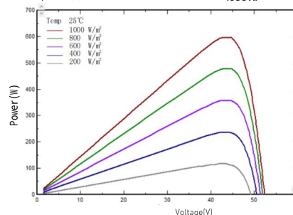
I-V/P-V Curve at Different Irradiation (600W)
