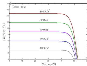
I-V/P-V Curve at Different Irradiation (625W)
