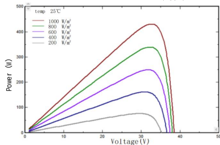
I-V/P-V Curve at Different Irradiation (435W)
