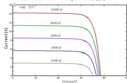
I-V/P-V Curve at Different Irradiation (435W)
