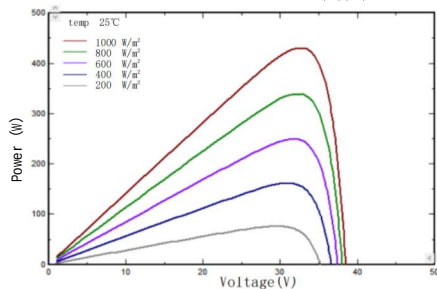
I-V/P-V Curve at Different Irradiation (460W)
