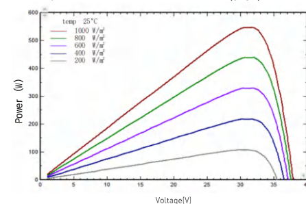
I-V/P-V Curve at Different Irradiation (545W)
