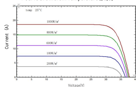
I-V/P-V Curve at Different Irradiation (545W)
